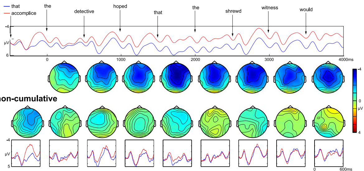
Fig. 4. Sustained negativity elicited in the comparison of the long-distance wh -dependency condition (red) and its control (blue), as reflected in waveform plots for midline electrode CZ, and topographic scalp maps based on mean voltage differences in successive 500 ms intervals. (A) Cumulative analysis, similar to Fiebach et al. [16] suggests that a sustained negativity persists throughout the wh -dependency. (B) Non-cumulative analysis, similar to King and Kutas [47], indicates that all words of the dependency do not contribute equally to the negativity. The topographic map for the first word of the cumulative analysis is not shown, since it is identical to the corresponding region in the non-cumulative analysis.
